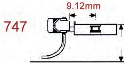
Medium Underset Shank
