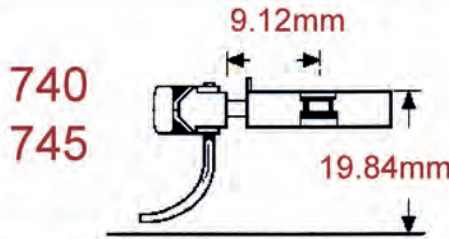
Medium Centerset Shank
