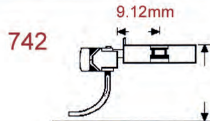
Medium Overset Shank
